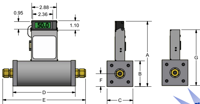
GM 1, GM 3 and GM 4 MASS FLOW METER DIMENSIONS
