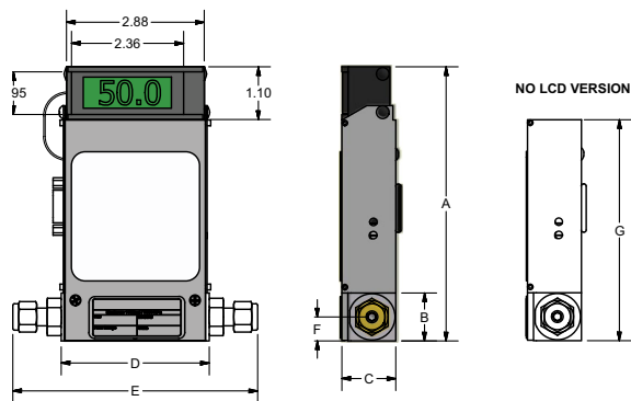
GM 1, GM 3 and GM 4 MASS FLOW METER DIMENSIONS
