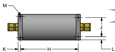
GM 1, GM 3 and GM 4 MASS FLOW METER DIMENSIONS
