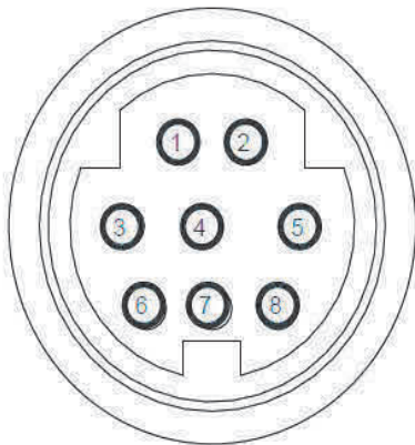
FIGURE 3: DPC 8-PIN Mini-DIN CONNECTOR CONFIGURATION
